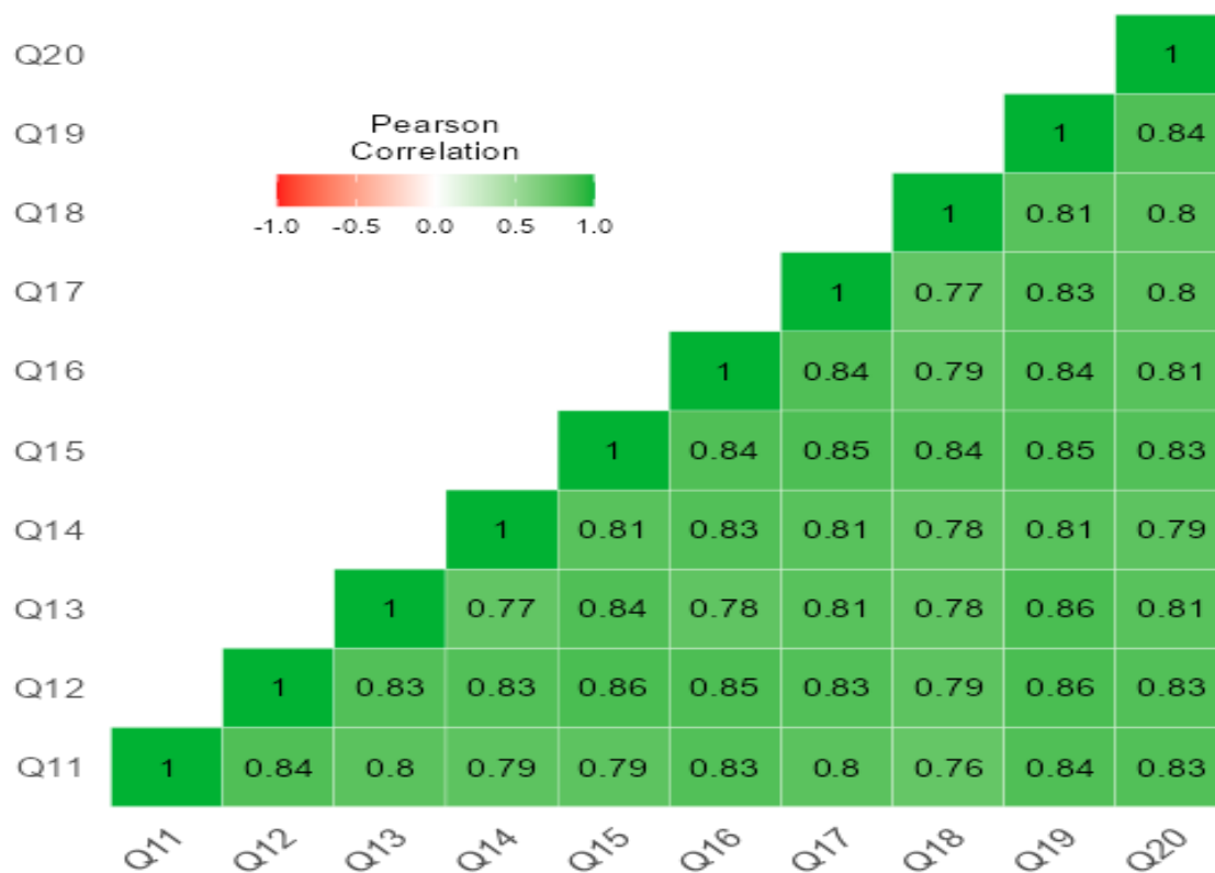
Correlation Heatmap
